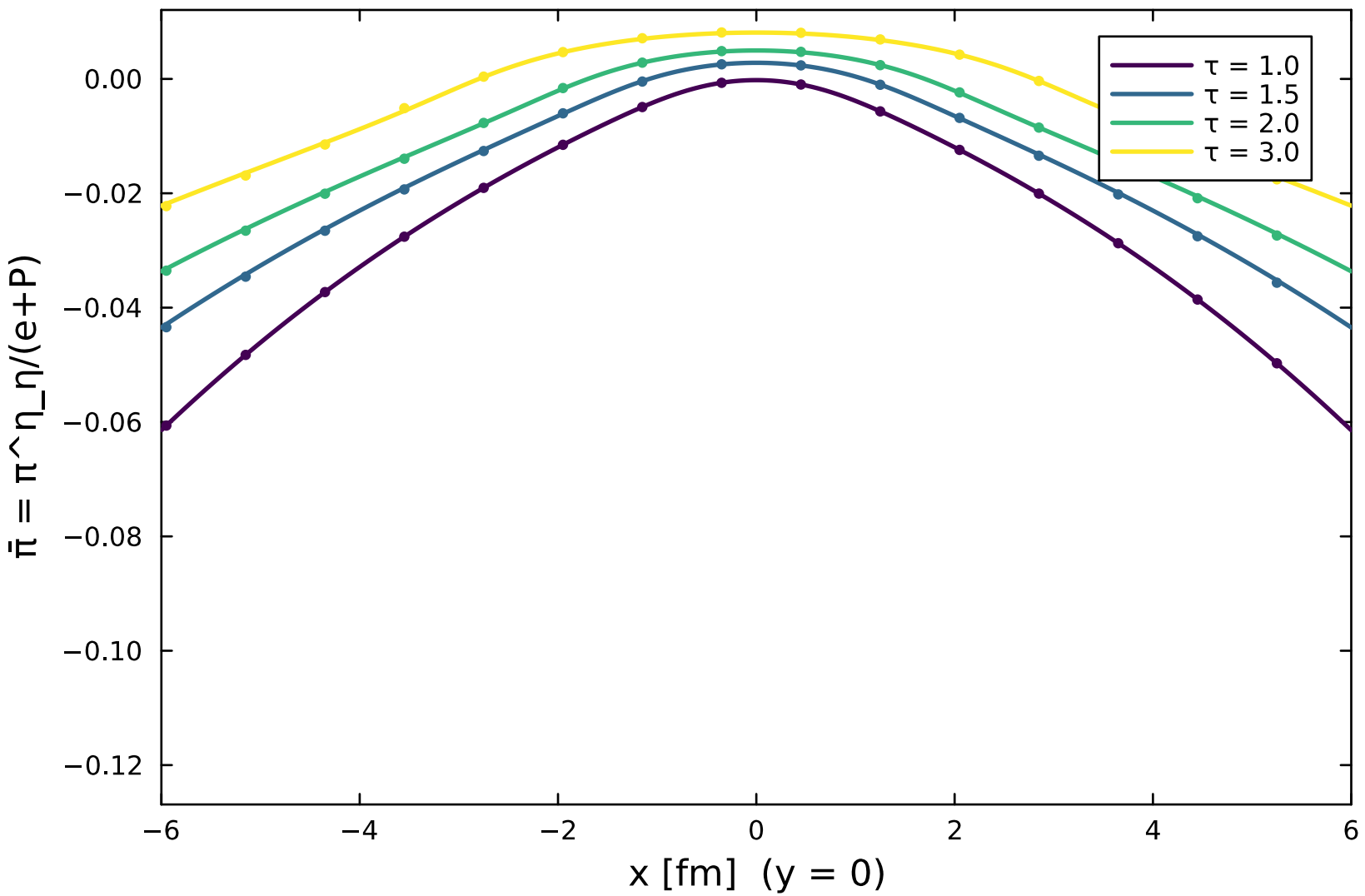
Gubser viscous \eta/s=0.02 — shear \bar{\pi} , lines semi-analytic
