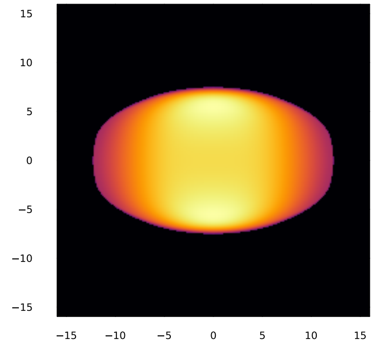
filament \tau = 8.0
