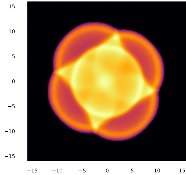
binary \tau = 8.0
