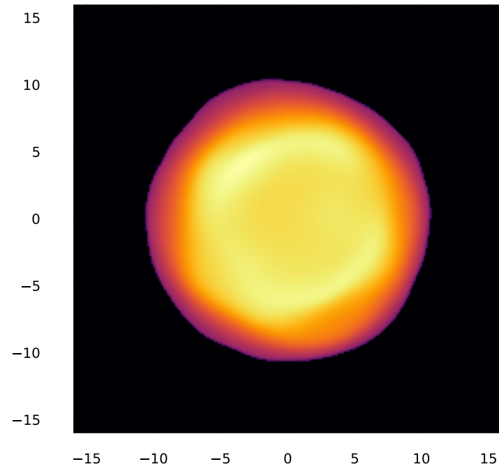
hotspots \tau = 8.0
