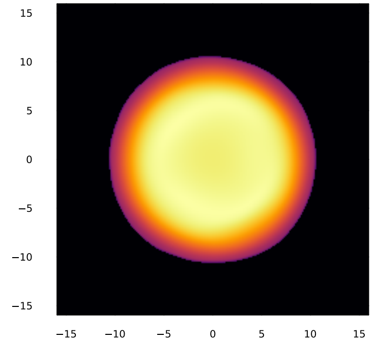
ring \tau = 8.0
