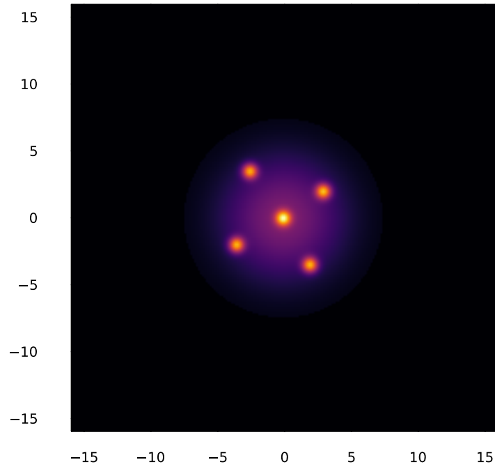
binary \tau = 0.4
