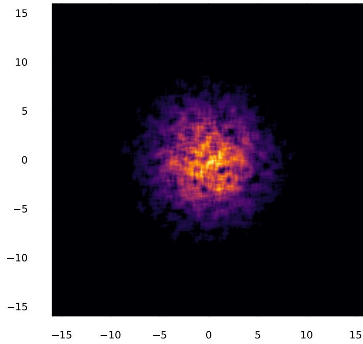
hotspots \tau = 0.4
