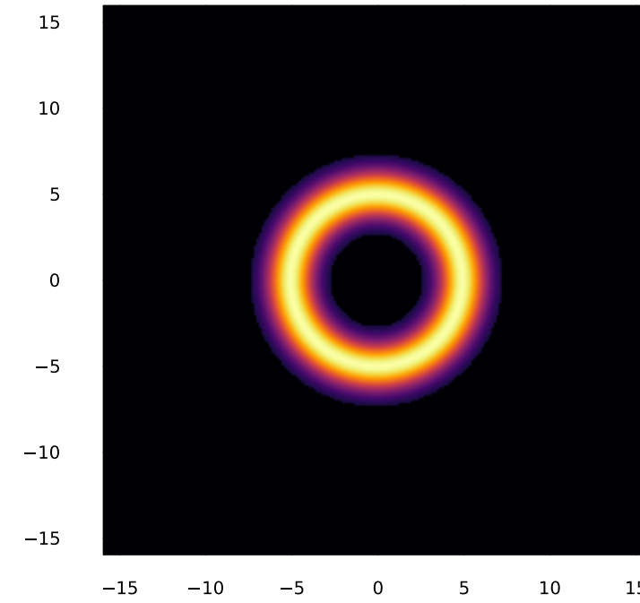
filament \tau = 0.4
