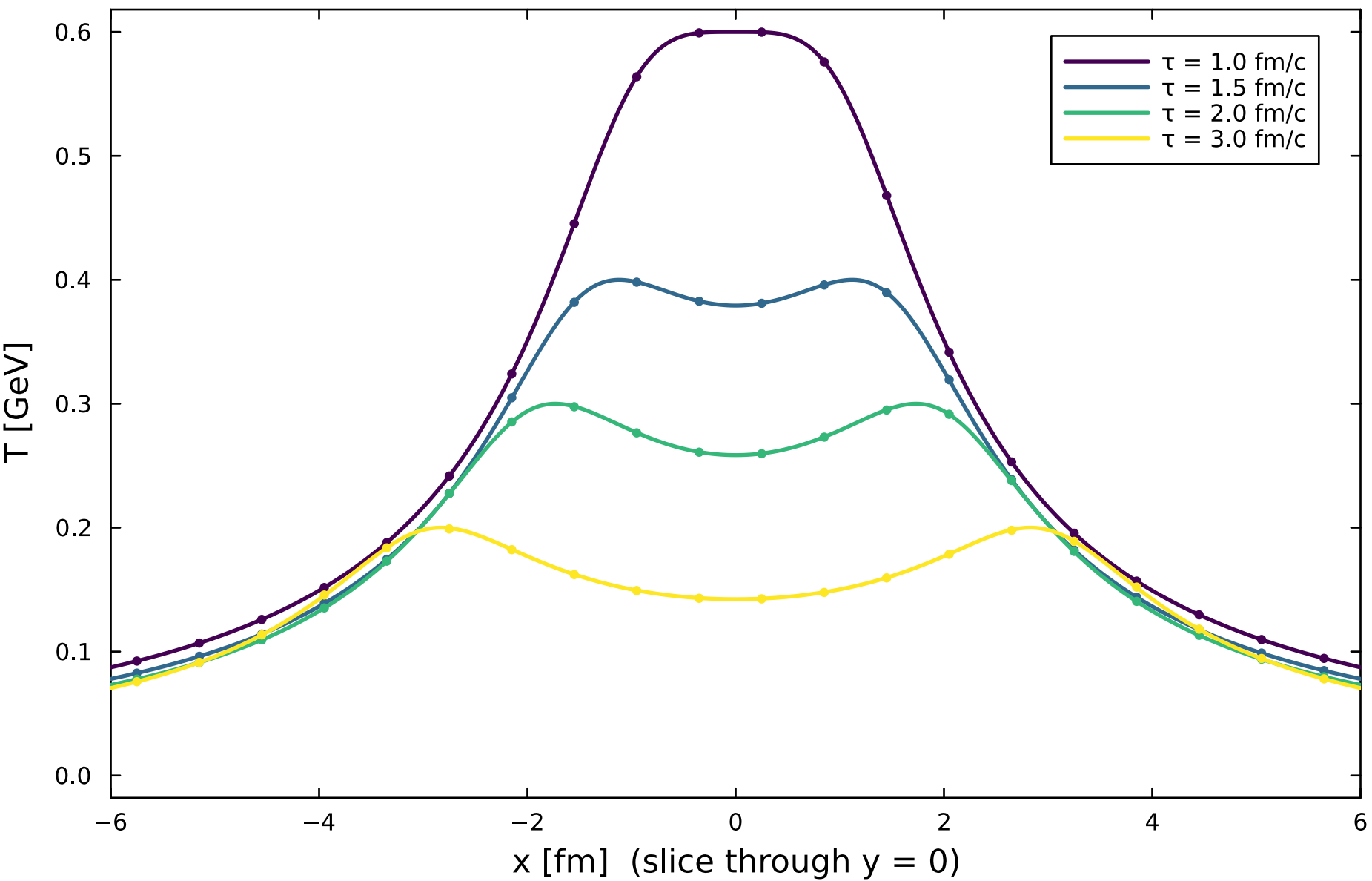
Gubser flow — solver (points) vs exact (lines)
