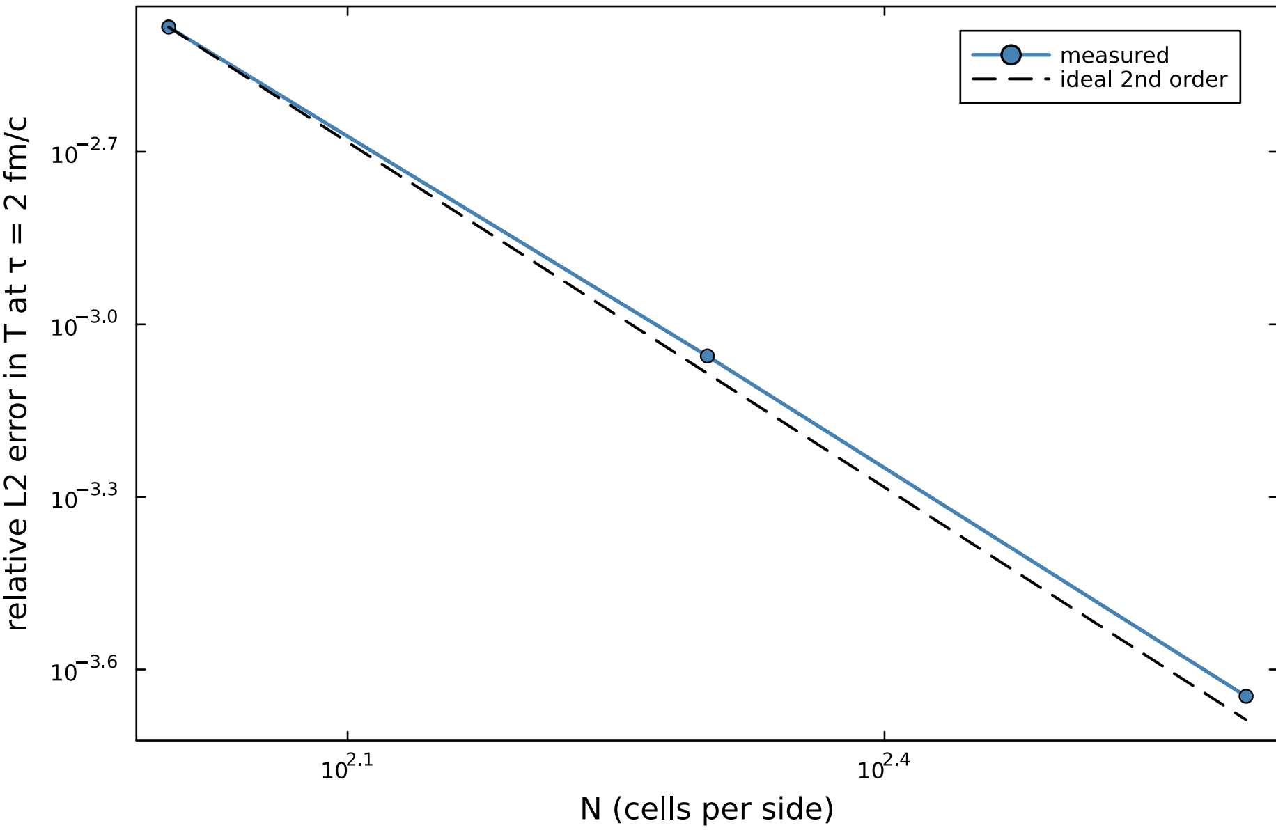
Second-order convergence to the exact solution
