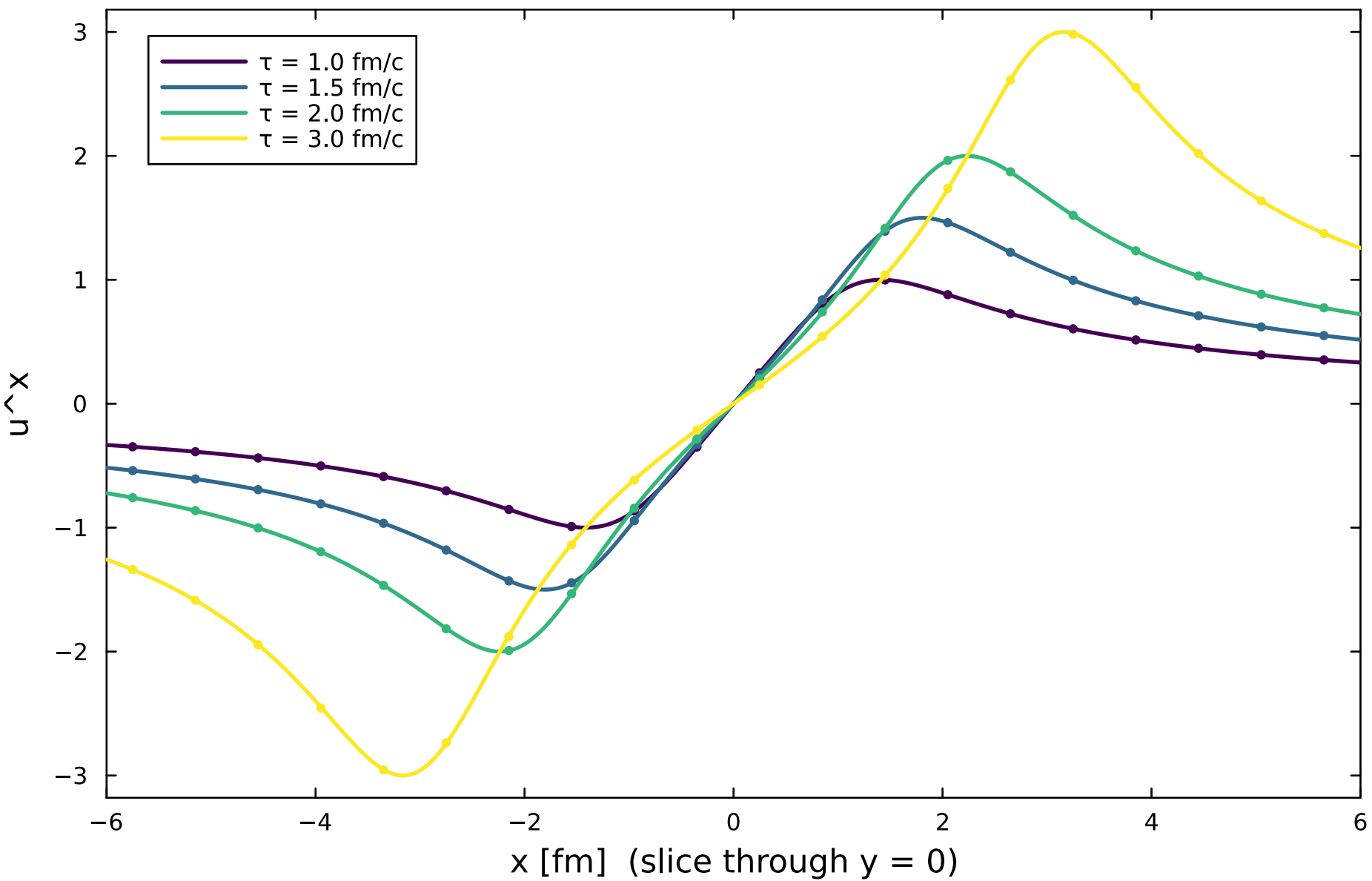
Radial flow — solver (points) vs exact (lines)
