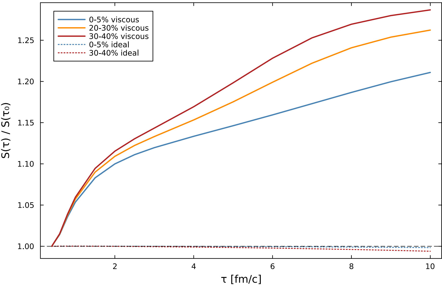
Entropy — viscous produces, ideal conserves
