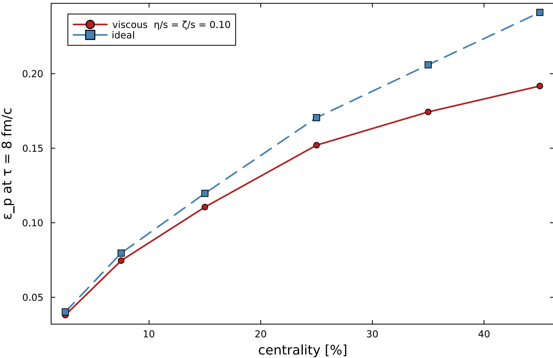
Elliptic flow vs centrality
