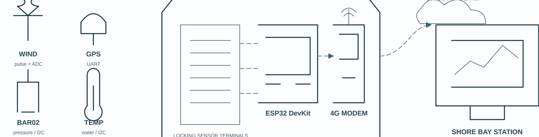
F — SUBSYSTEM INTERCONNECTION / DATA FLOW
