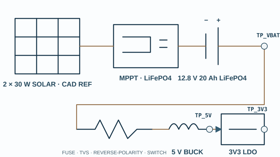
G — POWER MANAGEMENT
