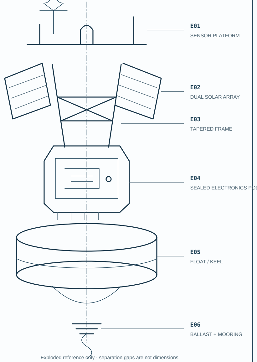
E — EXPLODED ASSEMBLY VIEW · NTS
