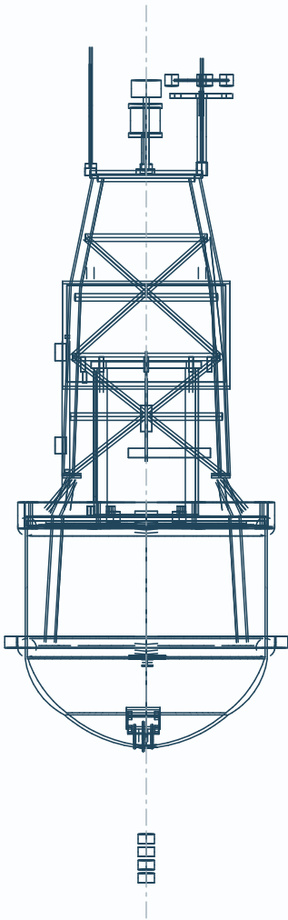
B — RIGHT ELEVATION
