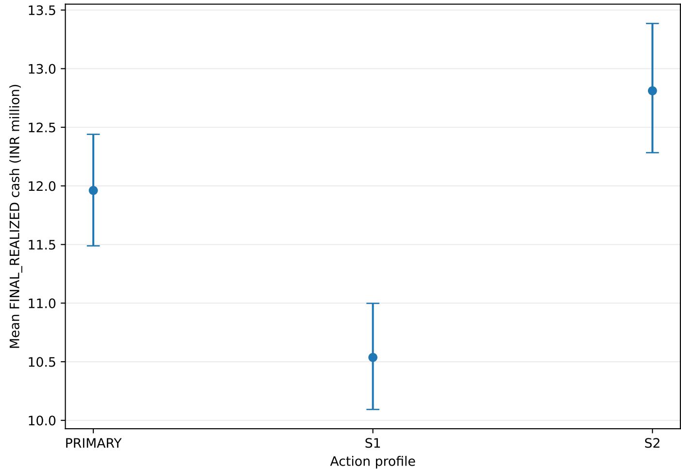
Action-profile robustness
