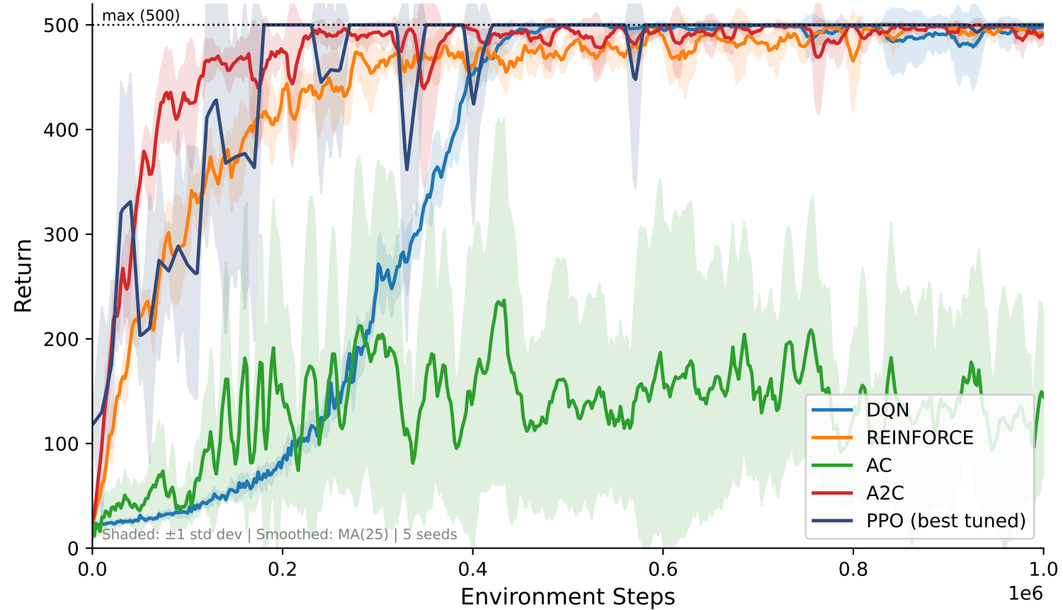
CartPole-v1: Algorithm Comparison
