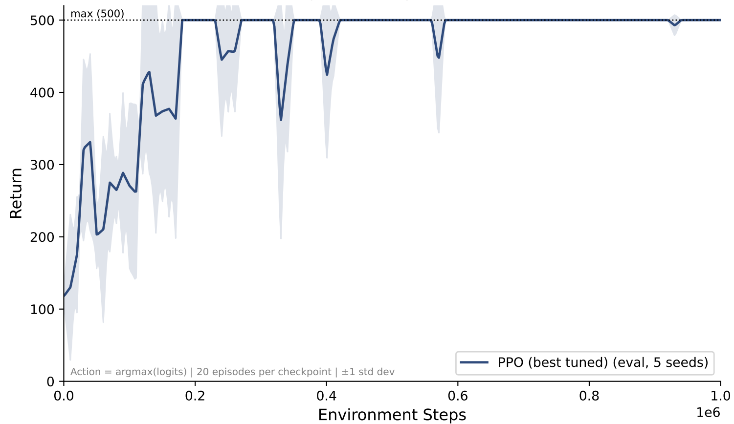
CartPole-v1: PPO (best tuned) Deterministic Evaluation
