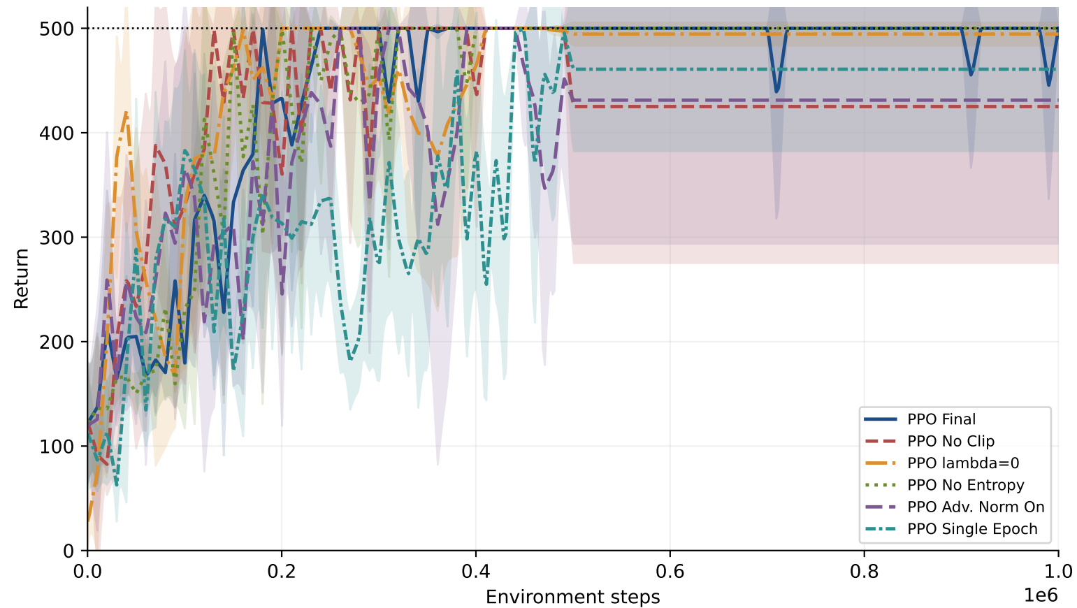
PPO ablation curves
