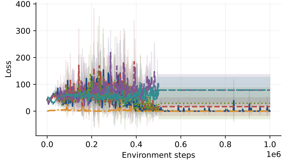
Value loss
