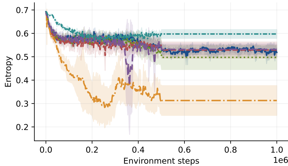
Policy entropy
