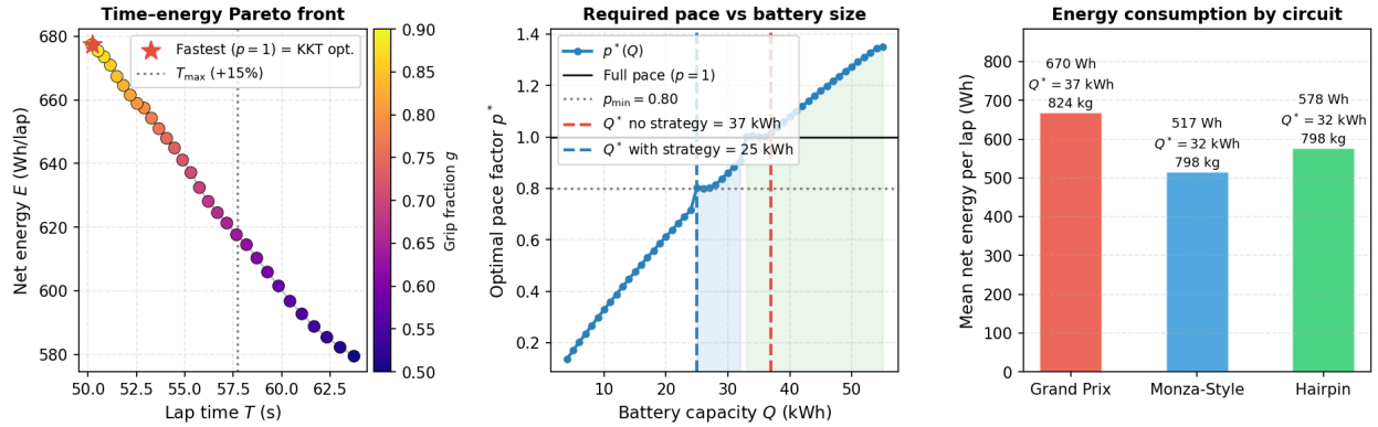
Figure 5: Race strategy and circuit comparison. Left: time–energy Pareto front; the fastest line within the competitive constraint ( T_{max} = +15\% ) minimizes battery usage at full pace. Middle: optimal pace factor p^*(Q) ; pace management reduces Q^* from 37 to 25 kWh (saving 60 kg). Right: mean energy per lap by circuit; the Monza-style circuit is 23% more efficient than the Grand Prix circuit due to lower curvature.
