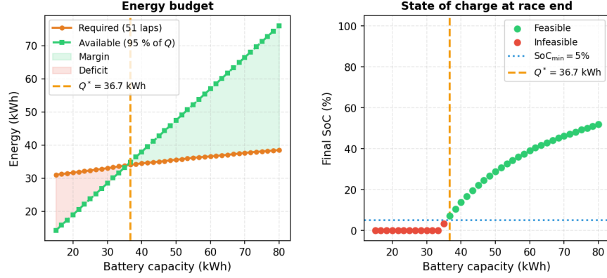
Figure 4: Battery sizing sweep. Left: required vs. available energy as a function of battery capacity, identifying the feasibility threshold Q^* \approx 37 kWh. Right: final state of charge at race end, showing a sharp transition between infeasible ( SoC \leq 0 ) and feasible regimes.
