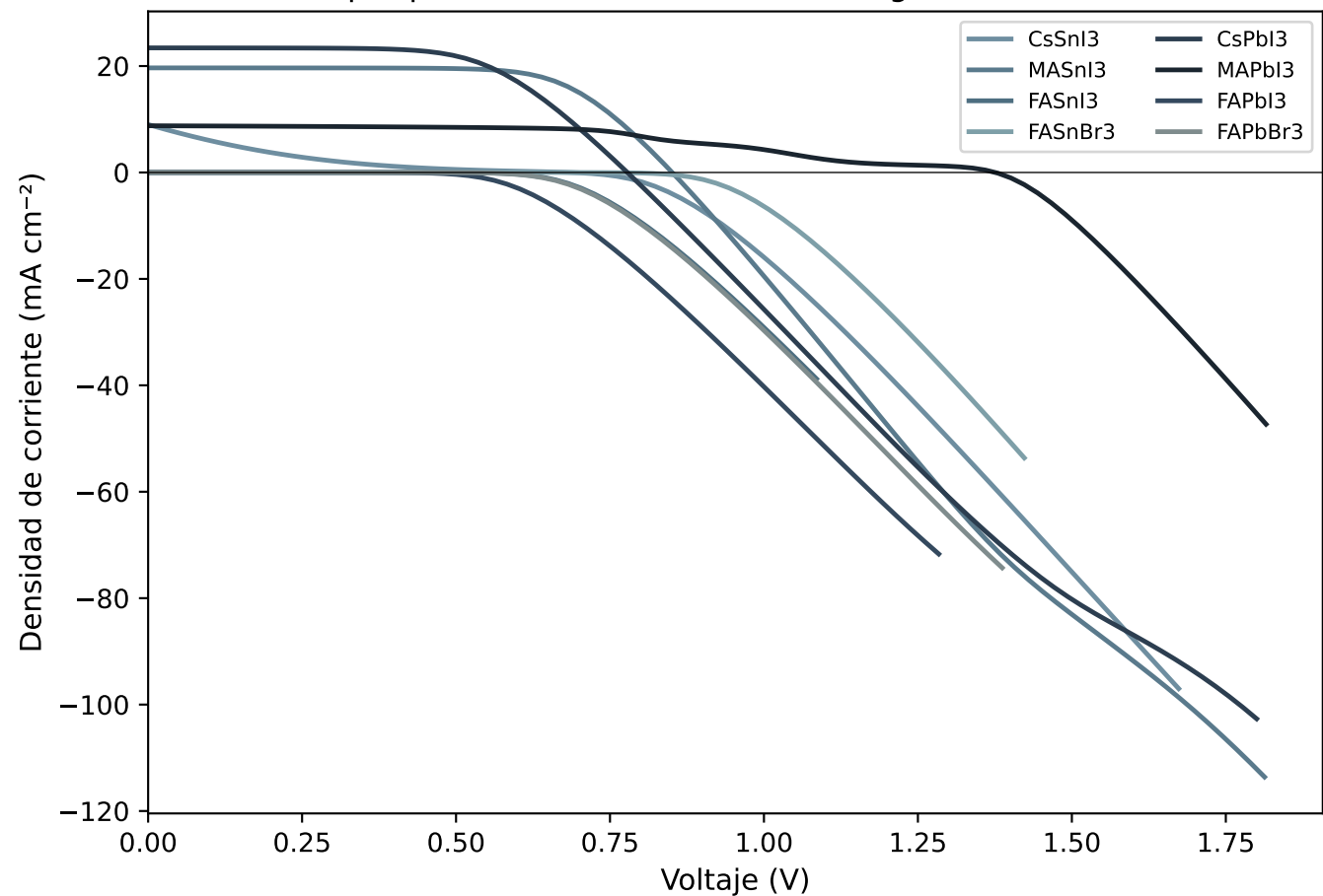
Top-8 perovskitas — drift-diffusion OghmaNano (DFT)
