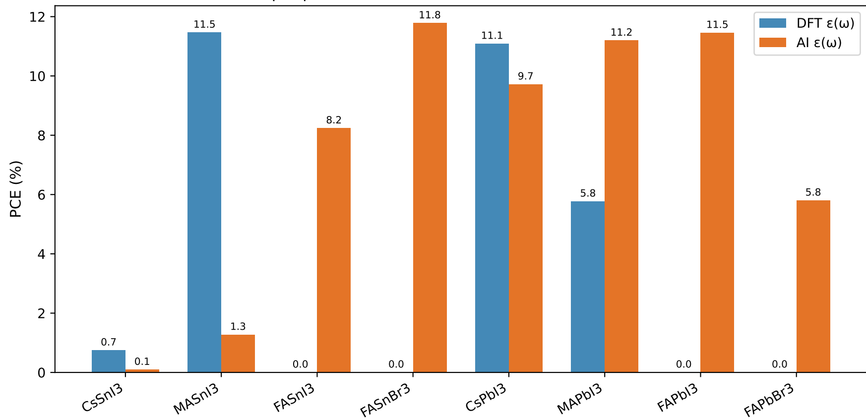
Top-8 perovskitas — PCE drift-diffusion (DFT vs AI \epsilon )
