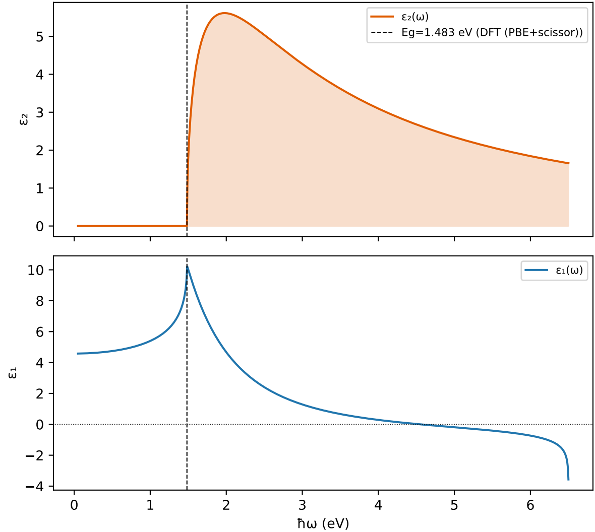
CsPbI3 — Función dieléctrica (Surrogate ( \epsilon_\infty=4.58 , Surrogate-ML (RF+GBR, \sigma=0.21 ); E_g=1.483 eV, DFT (PBE+scissor)))
