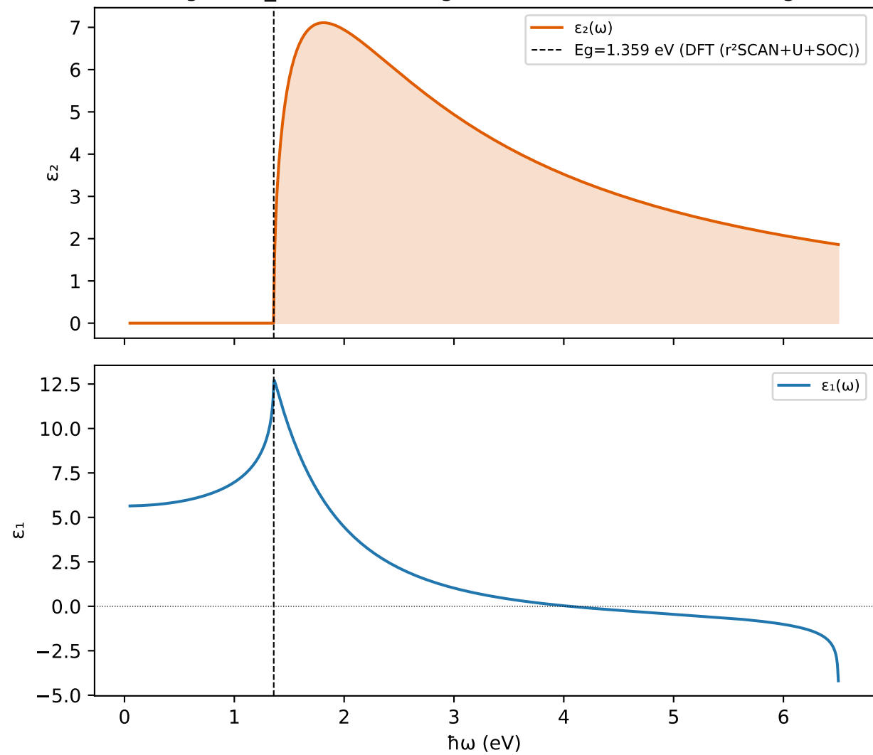
CsSnI3 — Función dieléctrica (Surrogate ( \epsilon_\infty=5.64 , Surrogate-ML (RF+GBR, \sigma=0.19 ); E_g=1.359 eV, DFT ( r^2 SCAN+U+SOC)))
