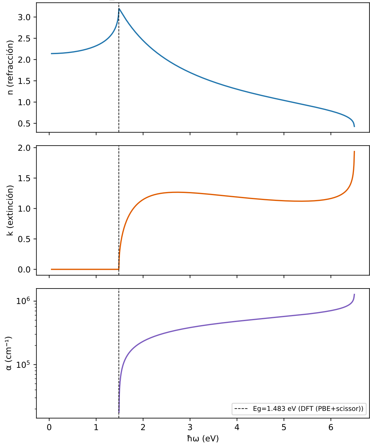
CsPbI3 — Espectro óptico (Surrogate ( \epsilon_{\infty} =4.58, Surrogate-ML (RF+GBR, \sigma =0.21); E_g =1.483 eV, DFT (PBE+scissor)))
