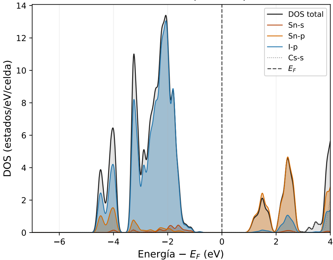
PDOS — CsSnI3 (r 2 SCAN+U)
