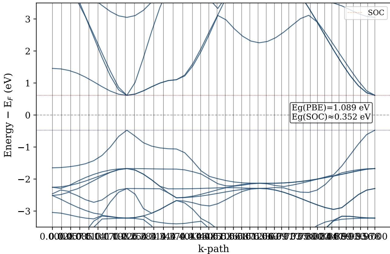
\alpha -CsPbI 3 | PBE + SOC overlay Gap = 1.089 eV direct at R=( \frac{1}{2}, \frac{1}{2}, \frac{1}{2} )
