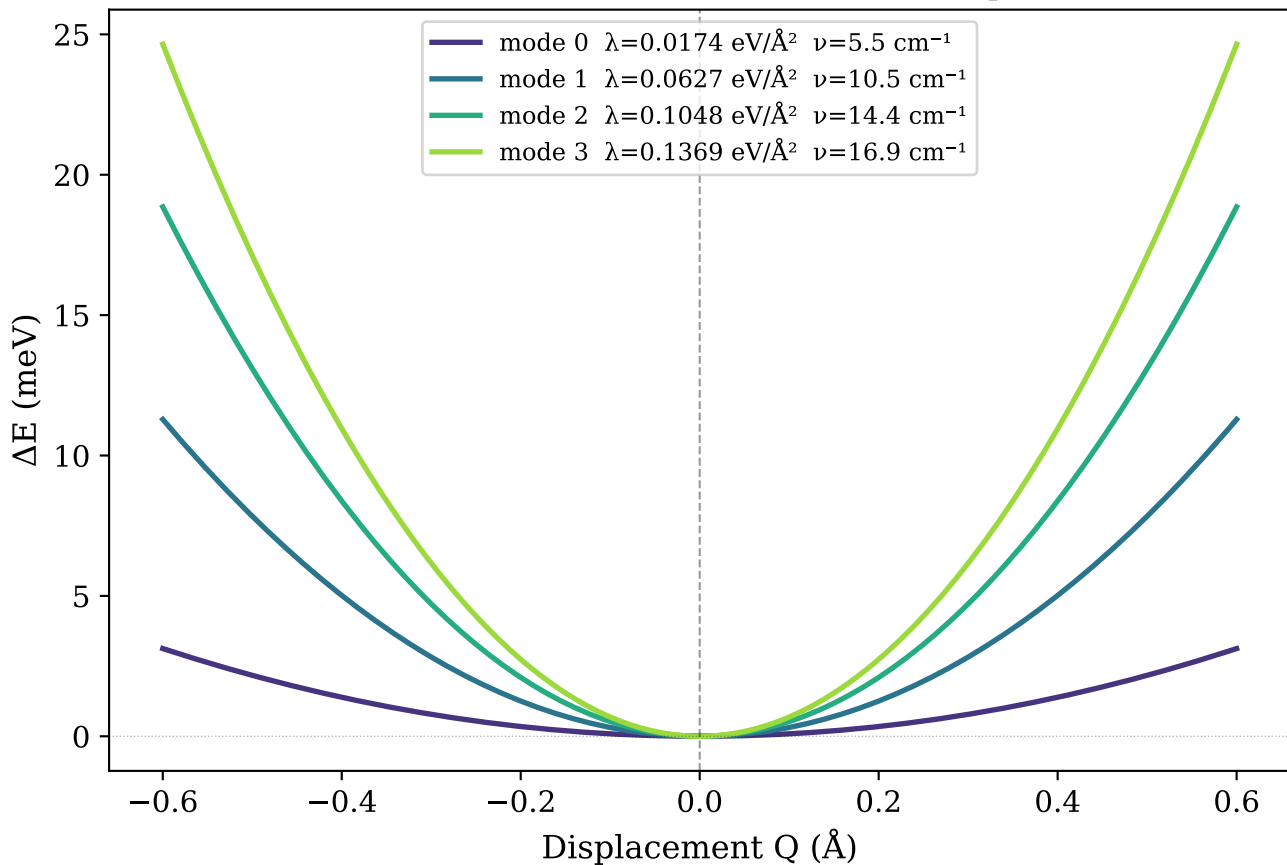
Harmonic PES — \alpha -CsPbI 3 soft modes ( \Gamma -point)
