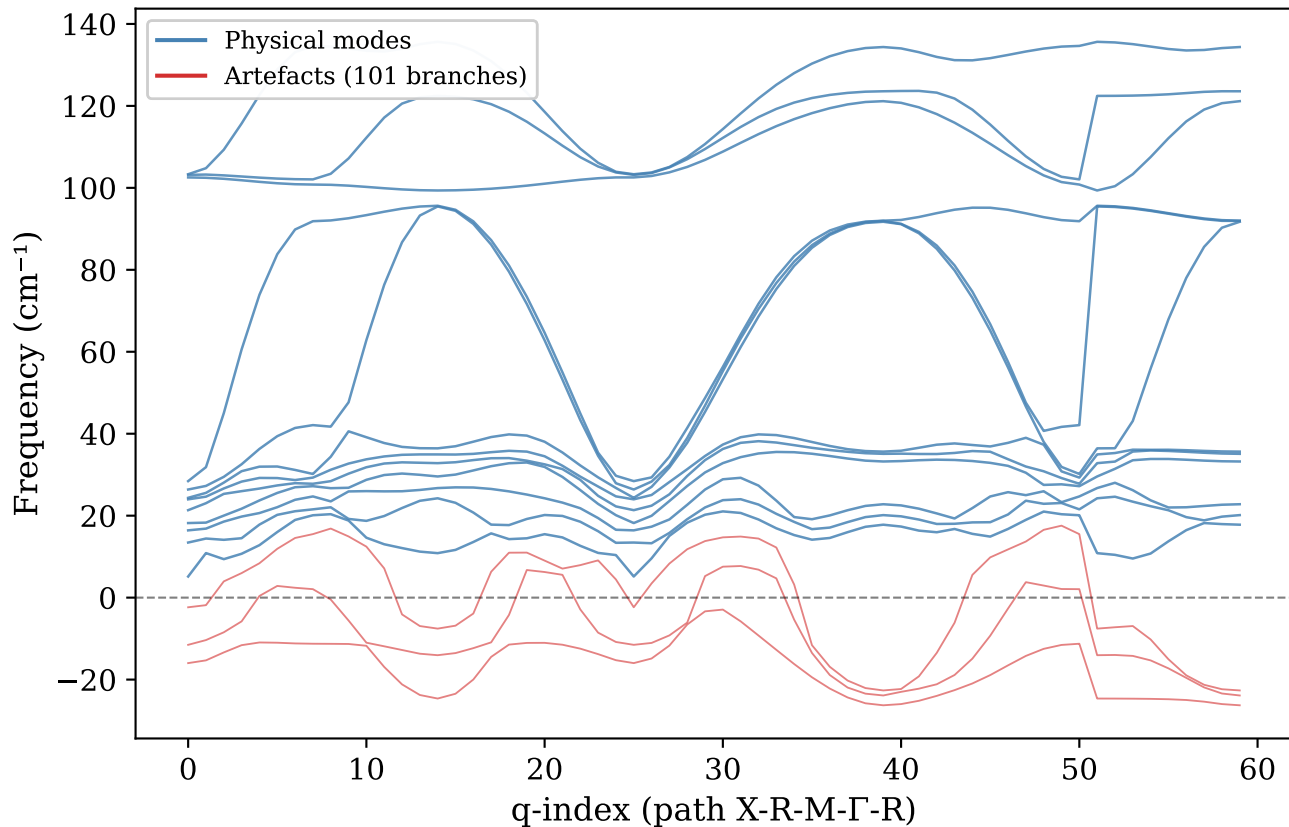
\alpha -CsPbI 3 | Phonon dispersion (ASE \Delta=0.05 Å) Optical range: 5.1-135.6 cm -1 | Acústicos: artefacto numérico
