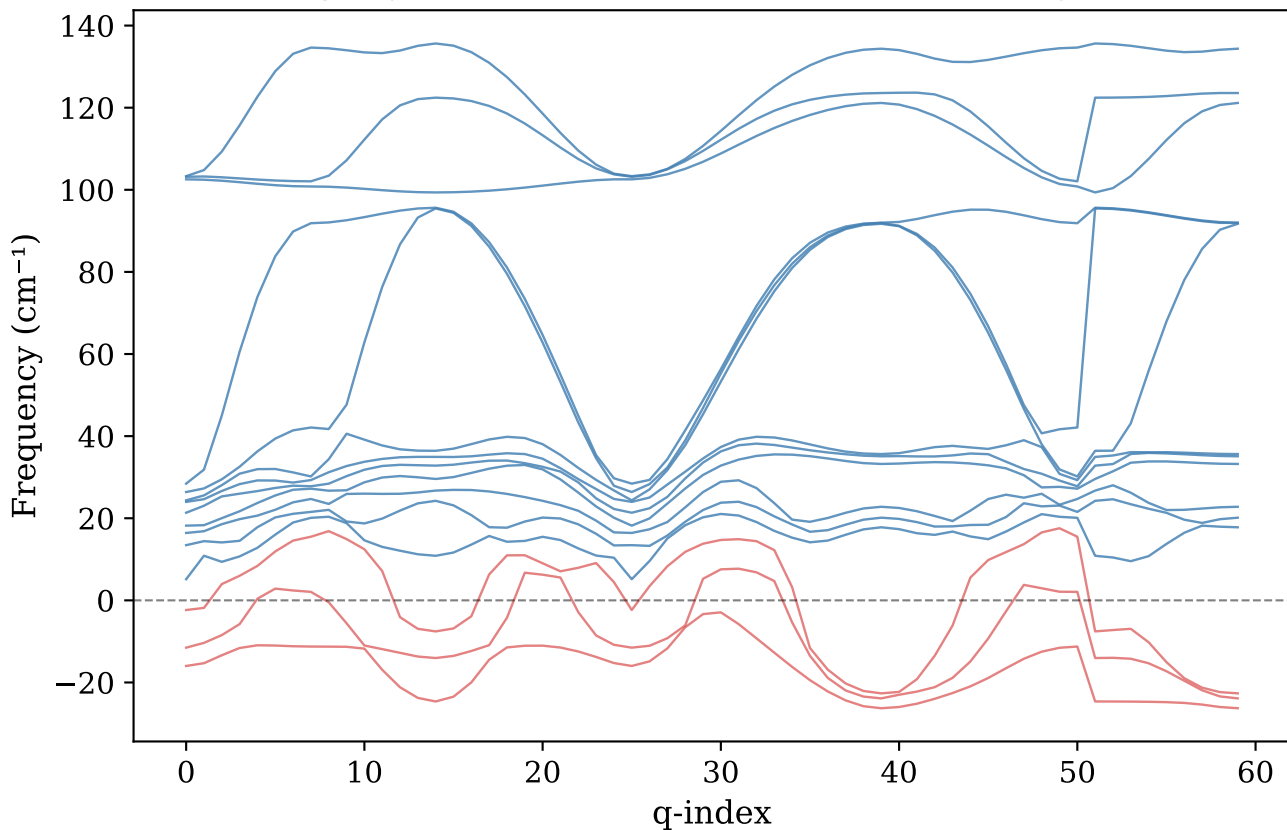
\alpha -CsPbI 3 | Phonon dispersion (ASE, \Delta=0.05 Å) Red=imaginary artefacts (101 branches < -10 cm -1 ), Blue=physical modes
