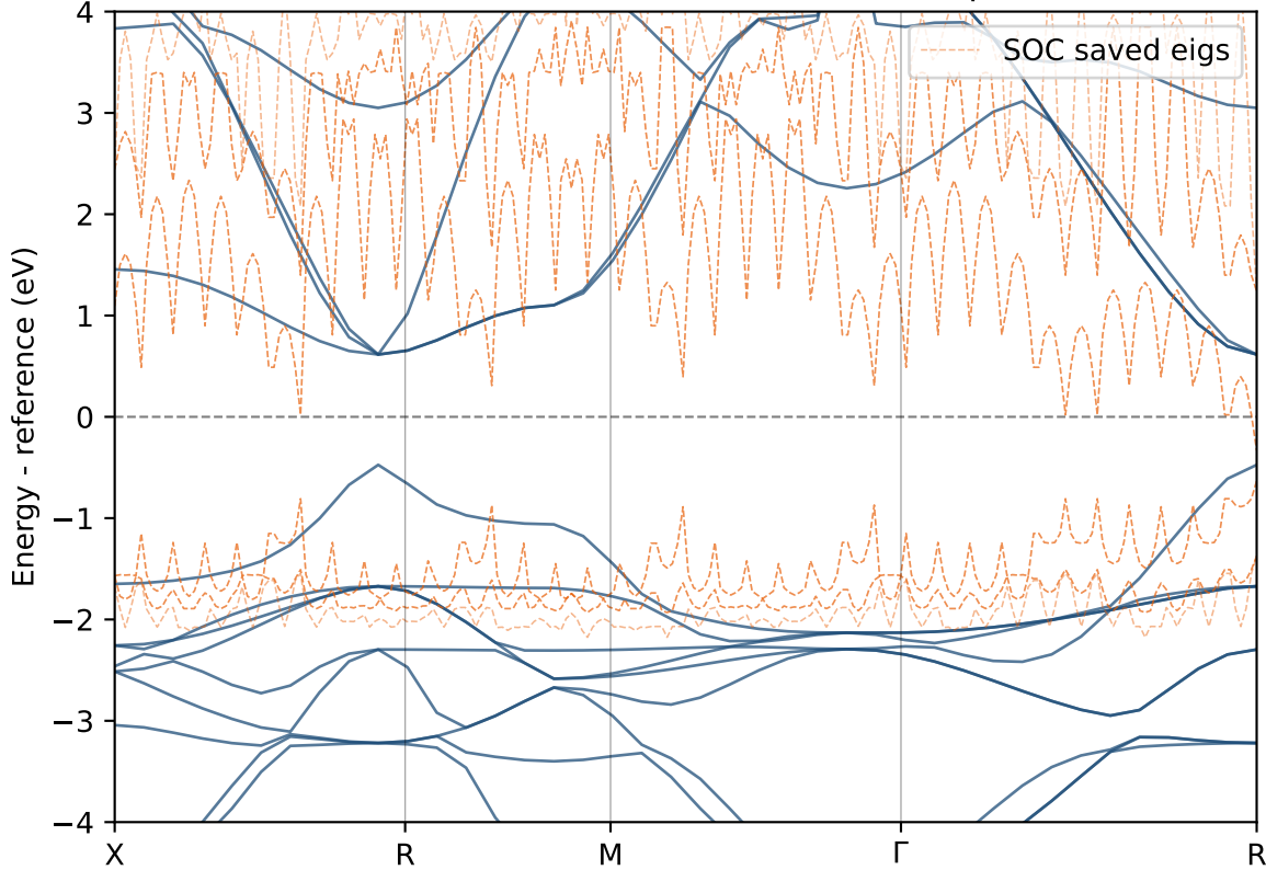
CsPbI 3 band structure from saved GPAW checkpoint-30/04/26
