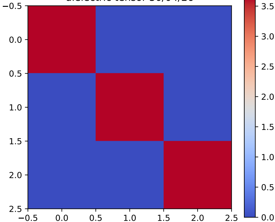
dielectric tensor-30/04/26
