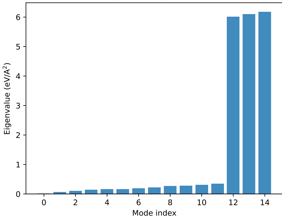
Hessian eigenvalue spectrum-30/04/26
