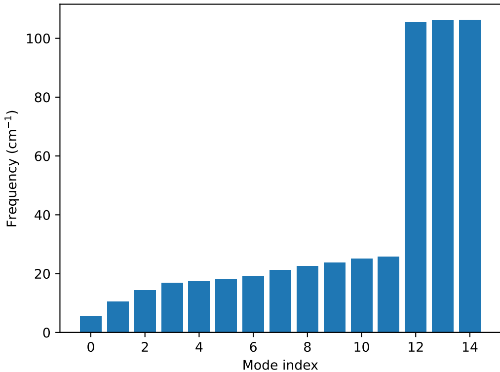
Gamma frequencies from mass-weighted Hessian-30/04/26
