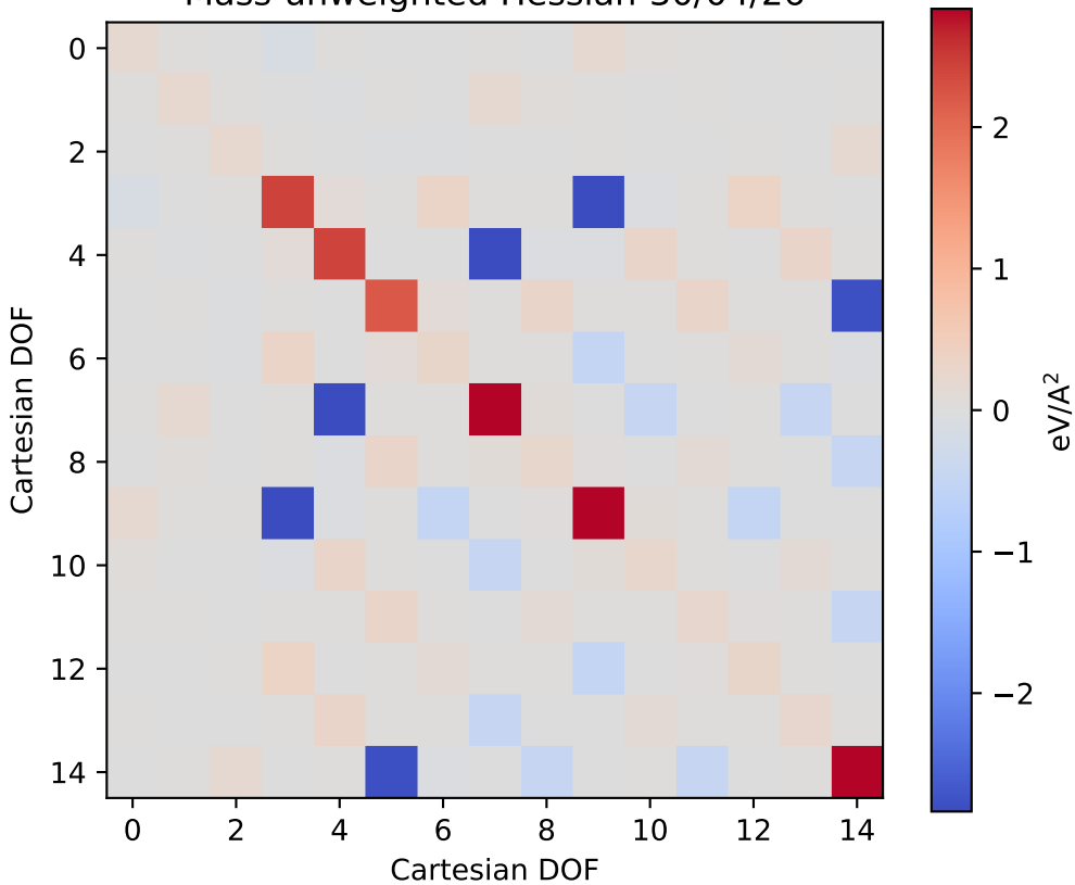
Mass-unweighted Hessian-30/04/26
