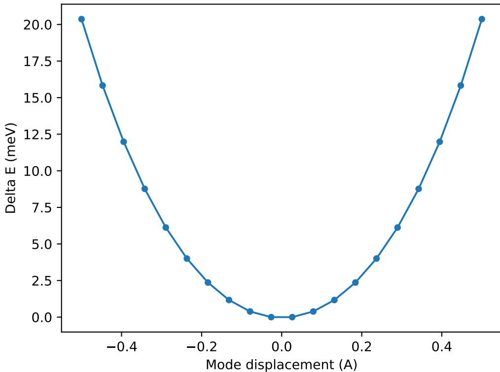
Potential-energy scan from saved NPY data-30/04/26
