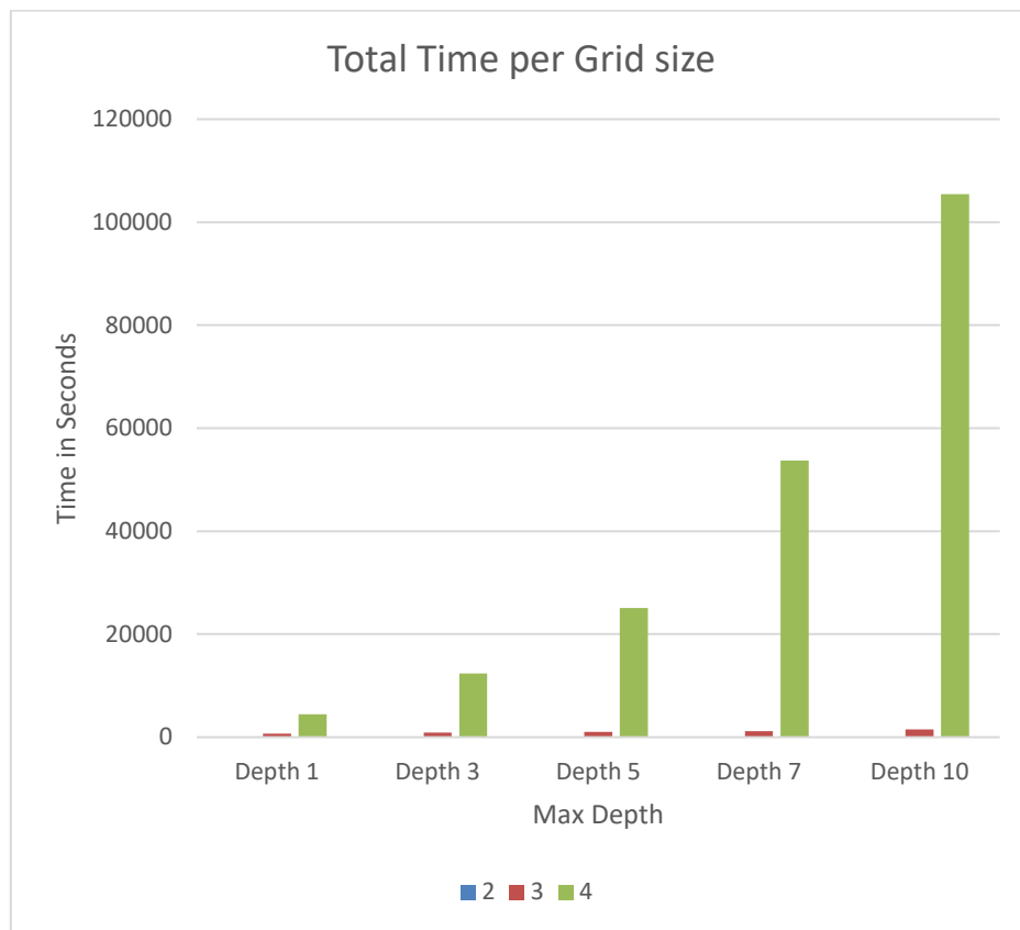
Figure 8 Total time per Grid Size graph
