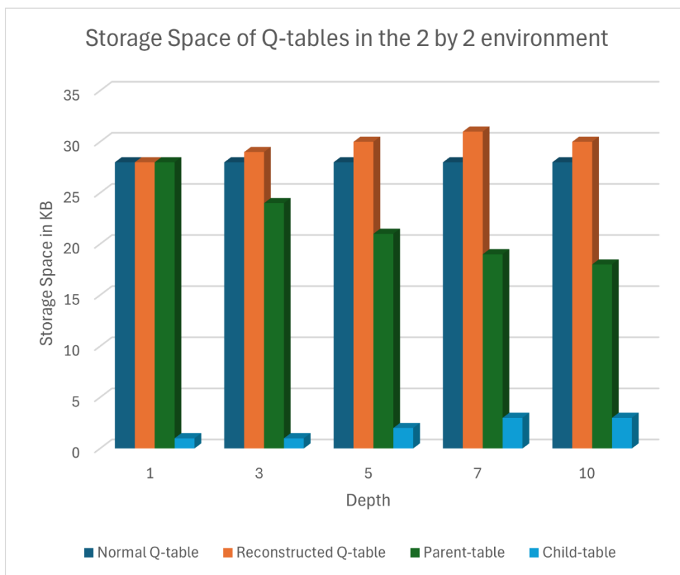
Figure 5 Storage Space of Q-table in 2 by 2 environment
