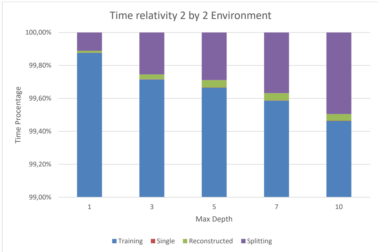
Figure 9 Time relativity 2 by 2 example
