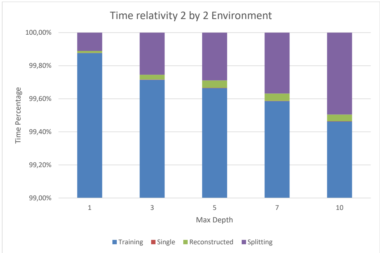
Figure 6 Time relativity 2x2 example
