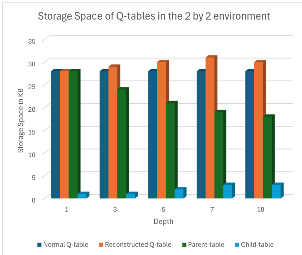
Figure 2 Storage Space of Q-table in 2x2 environment
