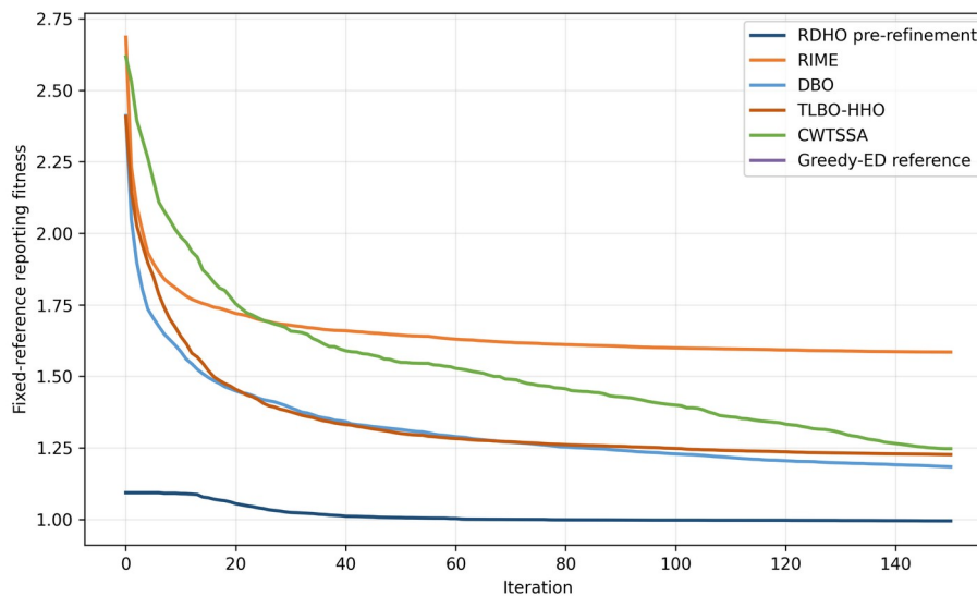
310 Fig. 2. Fixed-reference reporting-fitness convergence over 150 iterations. 311
