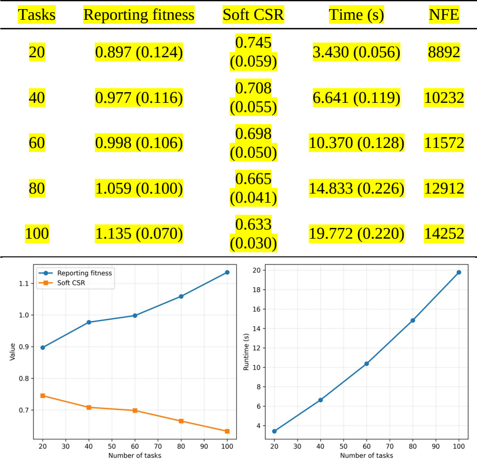
Fig. 9. Reporting fitness, soft CSR and runtime versus task count.
