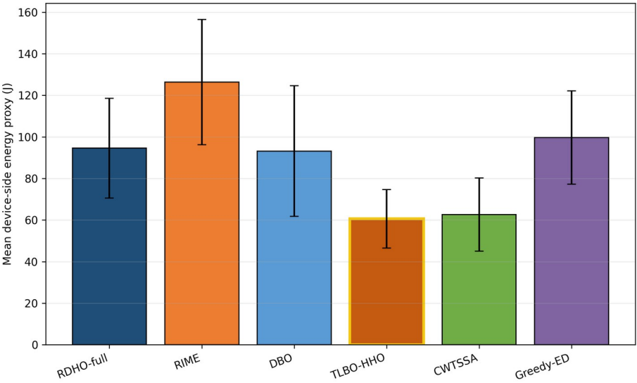
Fig. 3. Mean device-side energy over 30 paired runs. TLBO-HHO is the energy leader; RDHO optimises energy as one component of the coupled reporting preference.
