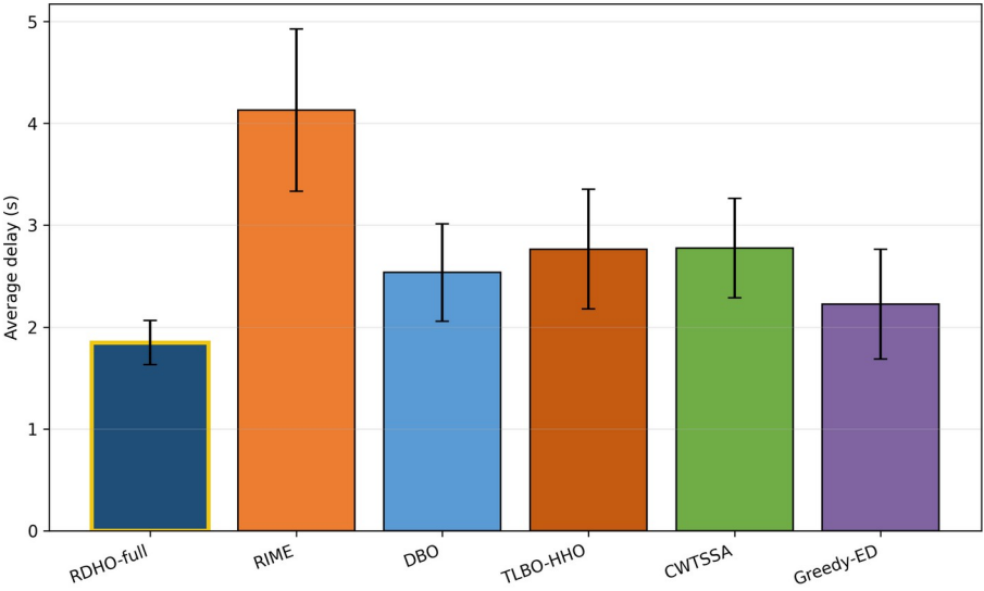
Fig. 4. Mean processing delay over 30 paired runs. RDHO-full has the lowest mean delay under the configured end-to-end procedures.
