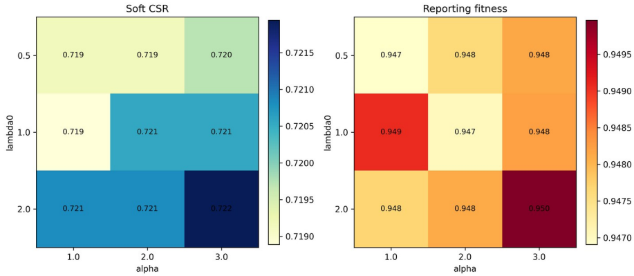
410 Fig. 11. Dynamic-penalty sensitivity heatmaps for soft CSR and reporting fitness.
