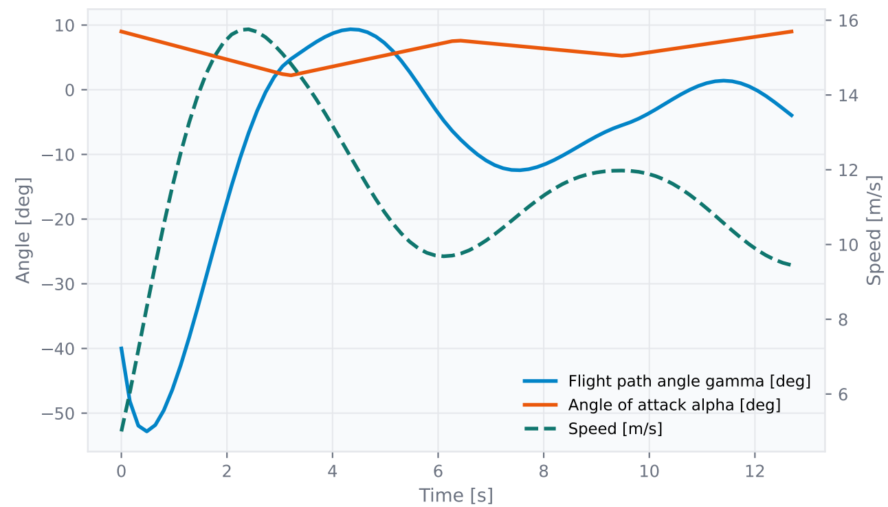
Flight States vs Time
