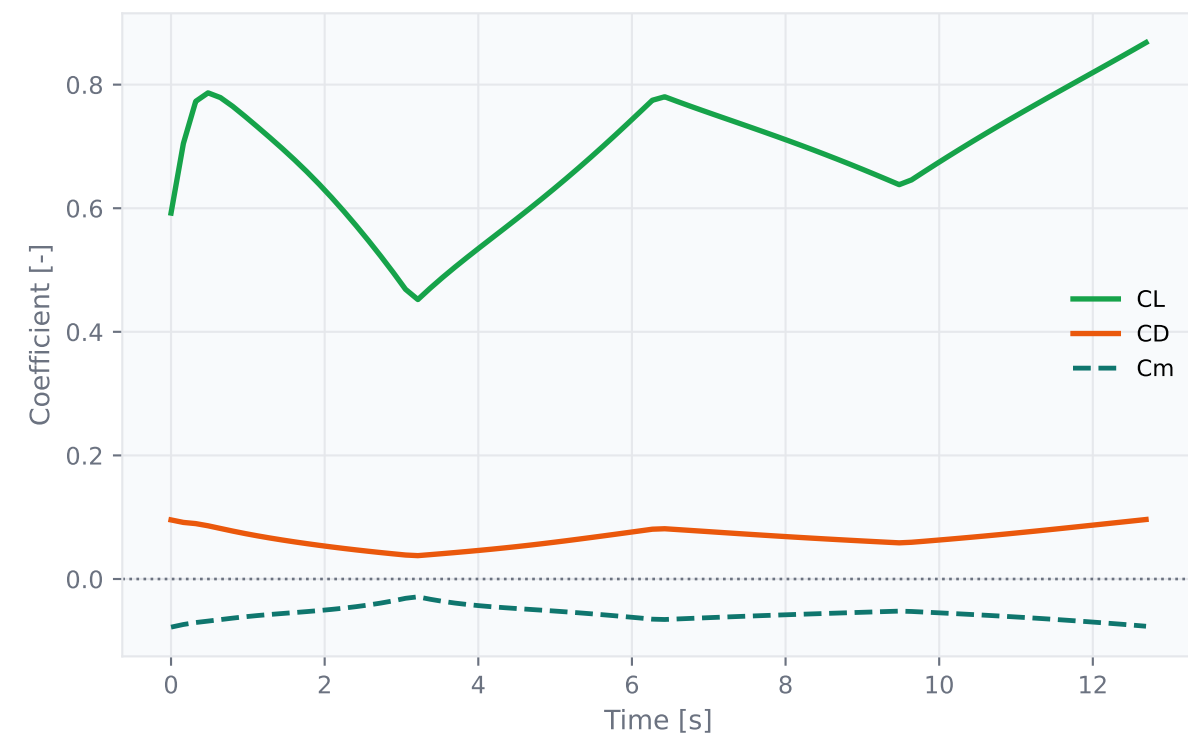
Aerodynamic Coefficients vs Time
