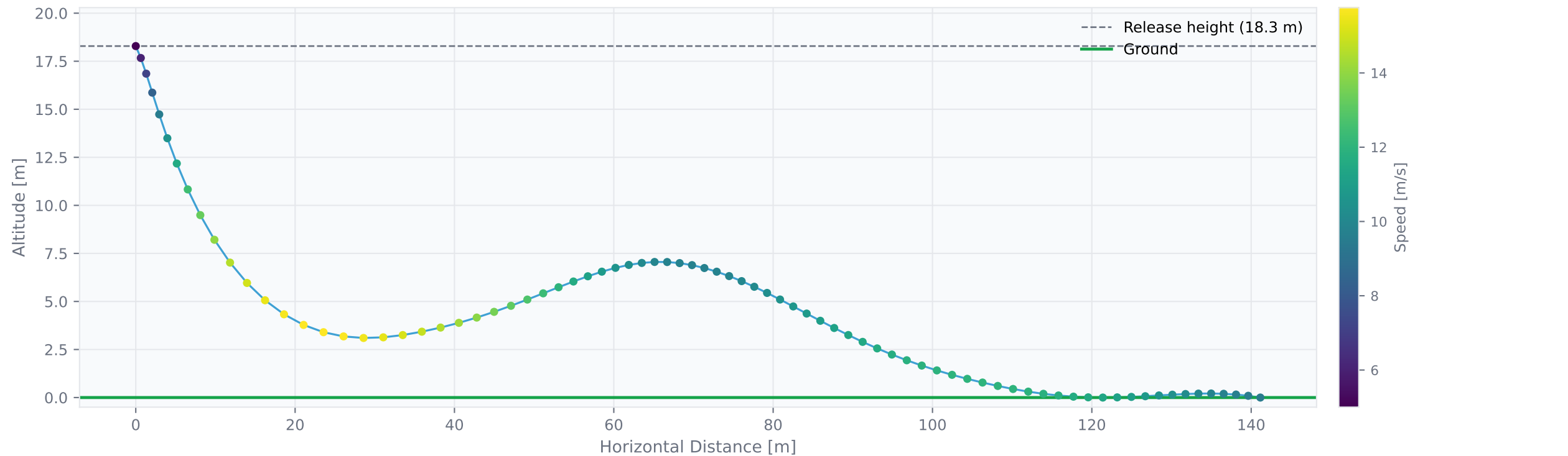
Optimized Drop-Glide Trajectory | T = 12.69 s, Range = 141.2 m
