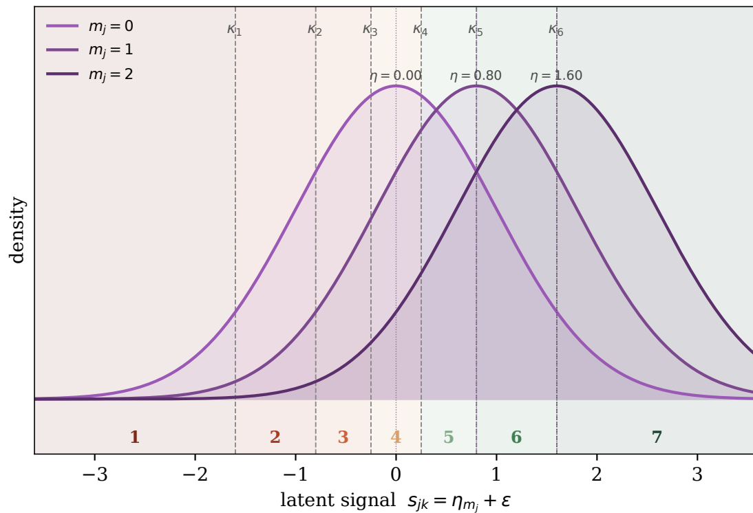
Ordered probit: latent signal \rightarrow Likert category
