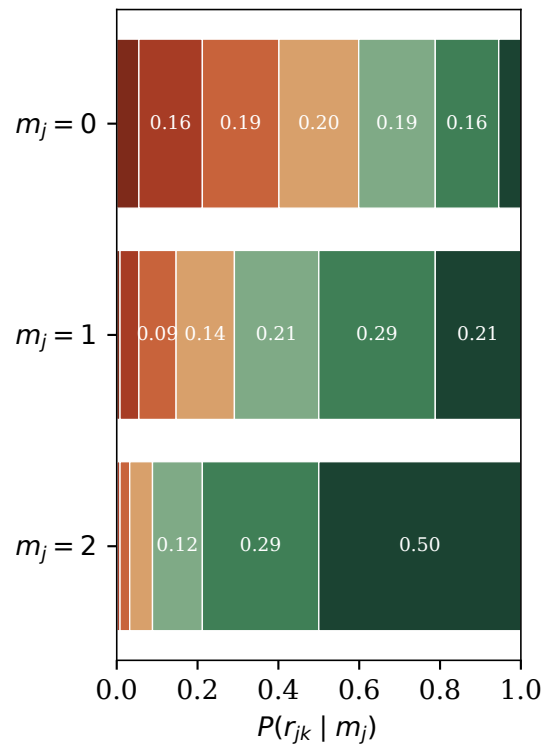
Implied category probabilities
