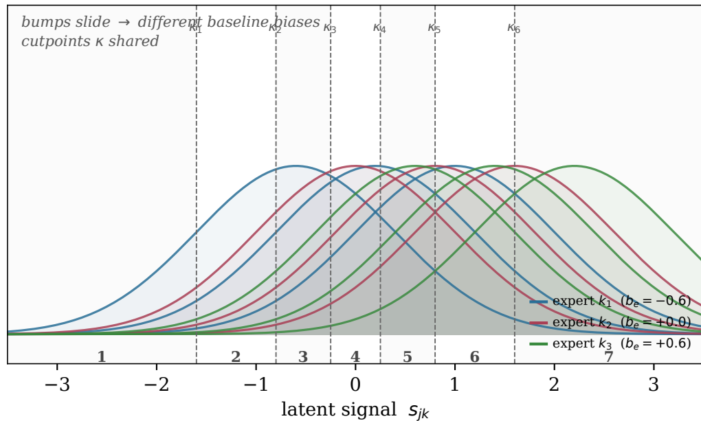
with per-expert b_e
