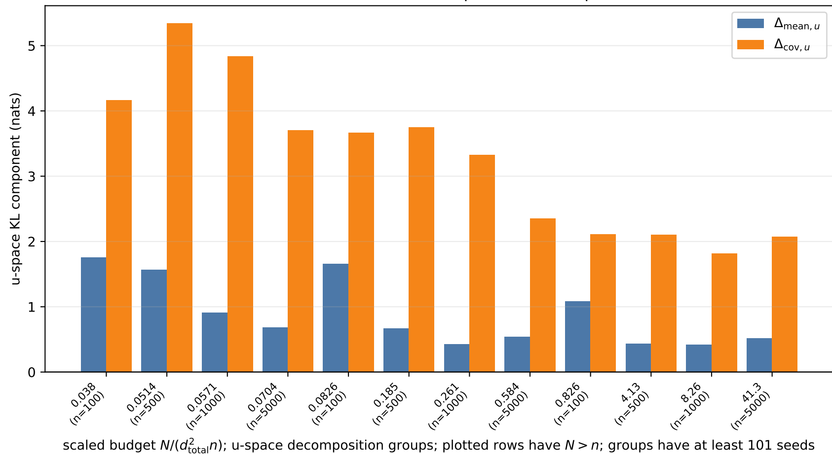
GNK Gaussian-NPE native u-space KL decomposition
