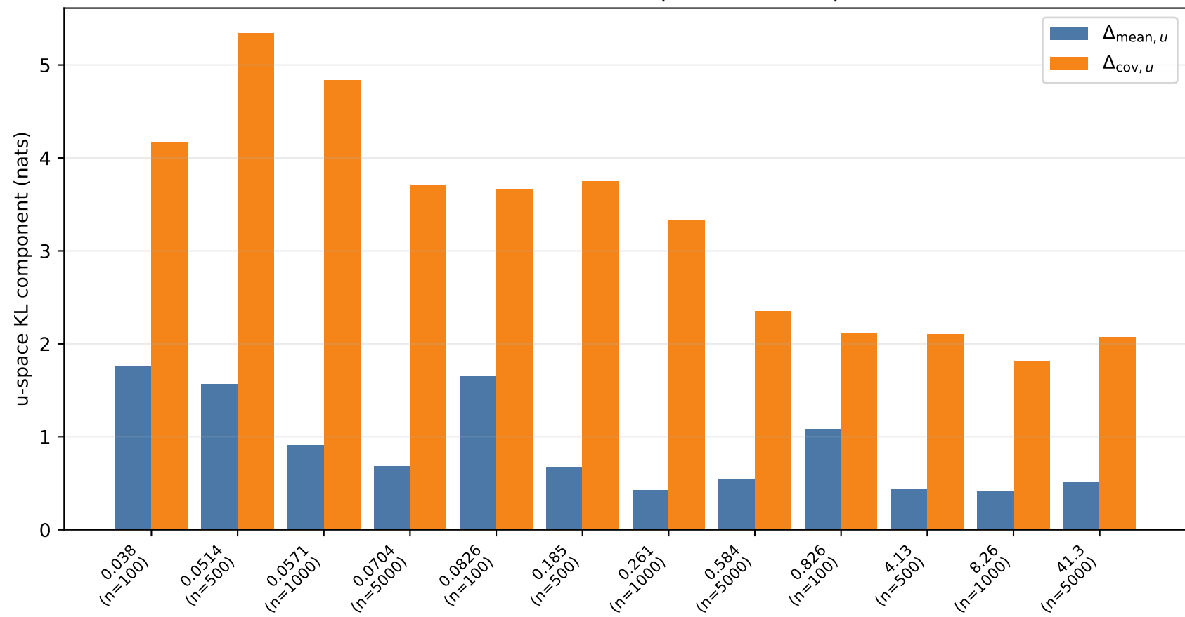
GNK Gaussian-NPE native u-space KL decomposition
