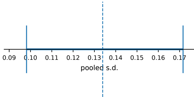
PRNPE-SMC-ABC
