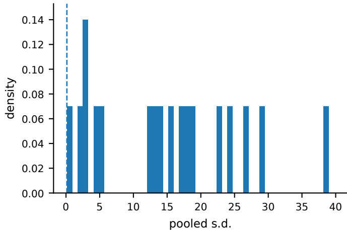
PRNPE-SMC-ABC
