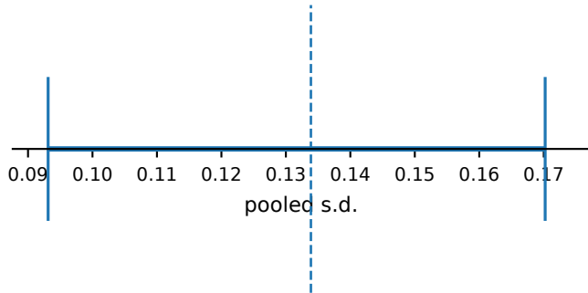
PRNPE-Random-Forest
