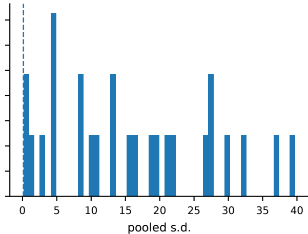
PRNPE-Random-Forest
