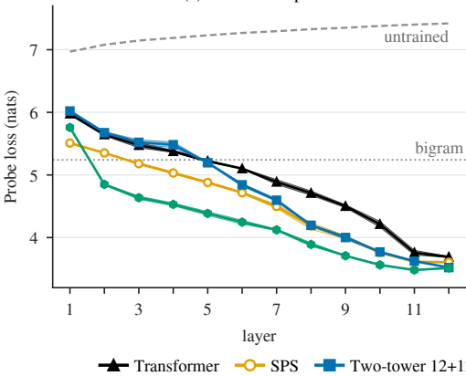
(a) Next-token probe
