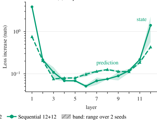
(b) Sequential 12+12: lesions
