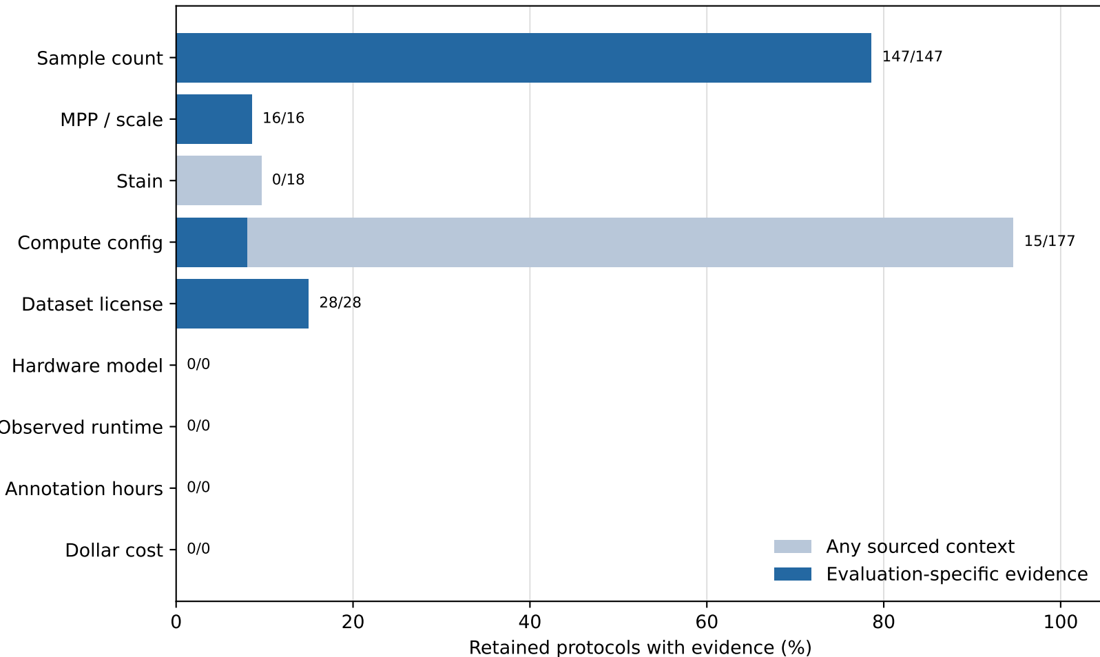
A. Evidence coverage (n=187)
