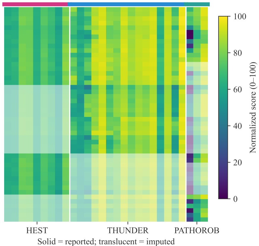
Completed matrix (latent interaction rank 1)
