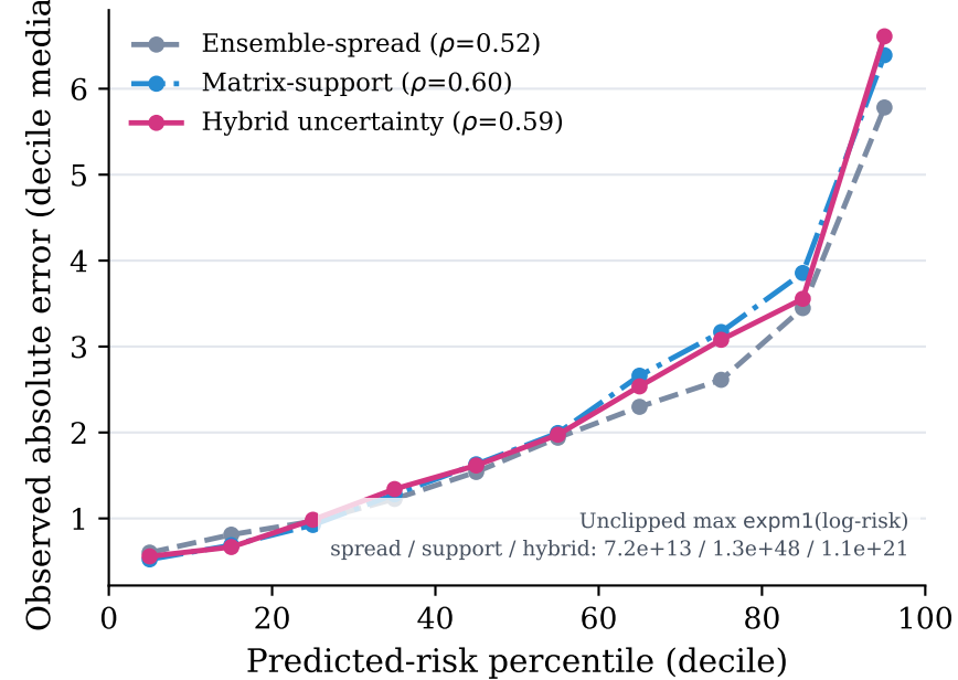
B Error-risk calibration
