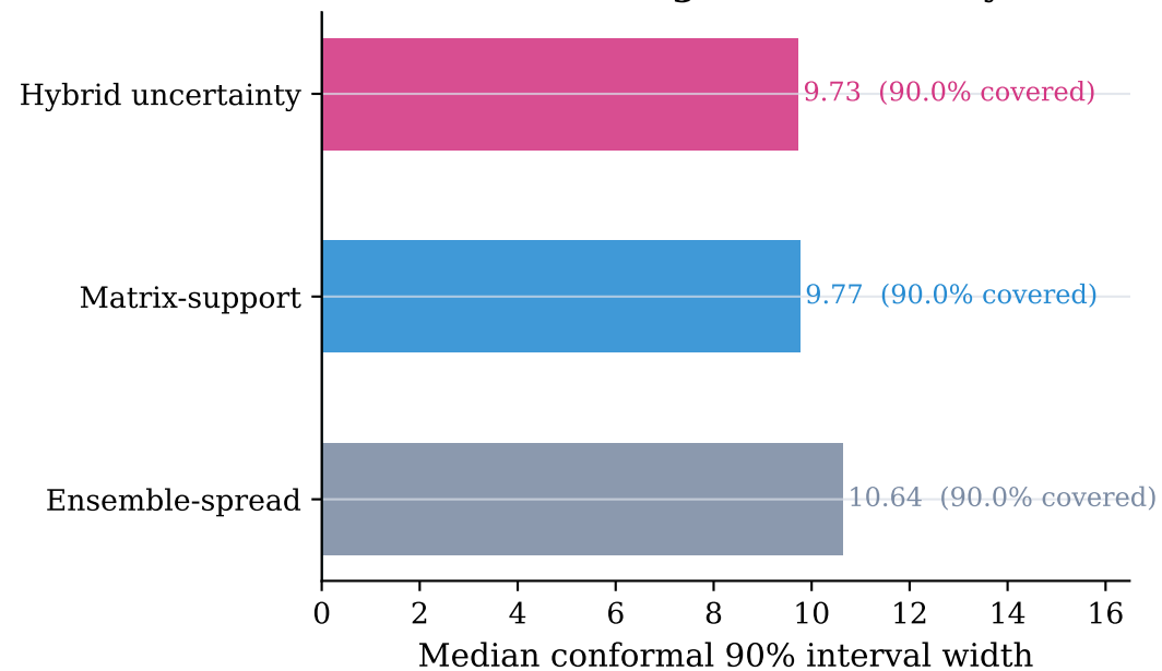
D Interval coverage and efficiency
