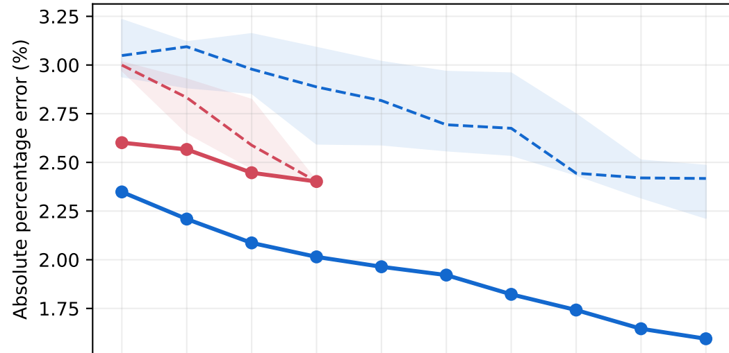
All-known parity — MEDAPE
