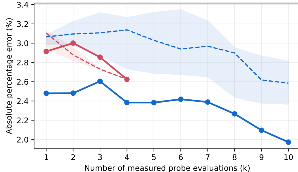
Held-out models — MEDAPE
