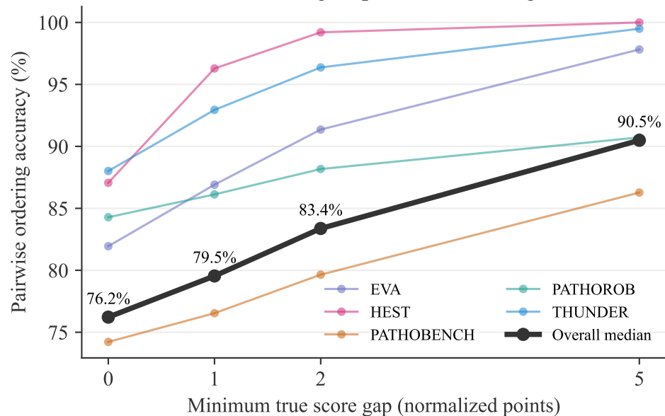
A Meaningful pairwise ordering
