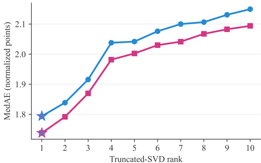
B Absolute-error view
