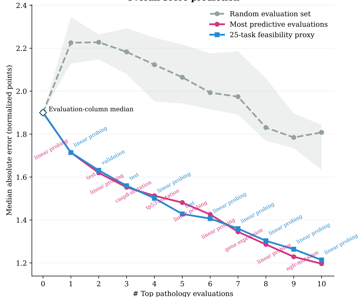
Overall score prediction
