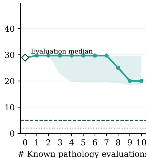
clip-b linear probing
